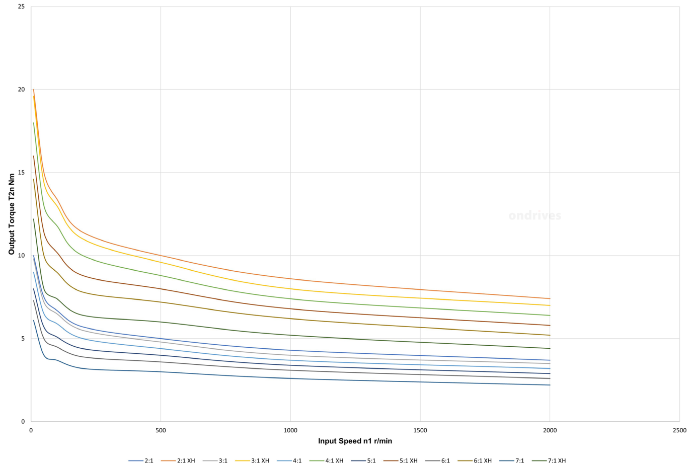
FF15 2:1 - 7:1 Series Parallel Offset Gearboxes
